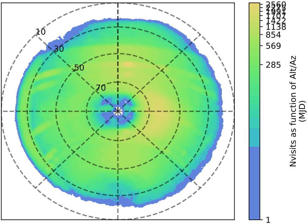
too_elab_heavy_r64_d2_ugrizy_v3.4_10yrs r: Nvisits as function of Alt/Az
