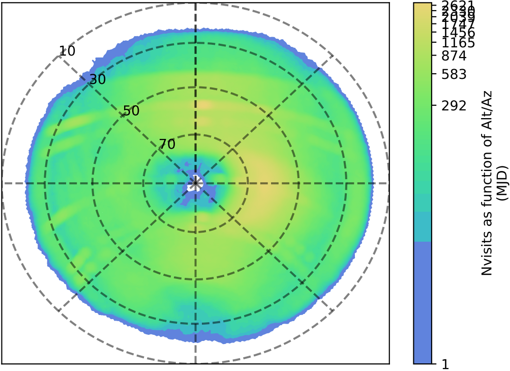
too_elab_heavy_r64_d2_ugrizy_v3.4_10yrs i: Nvisits as function of Alt/Az
