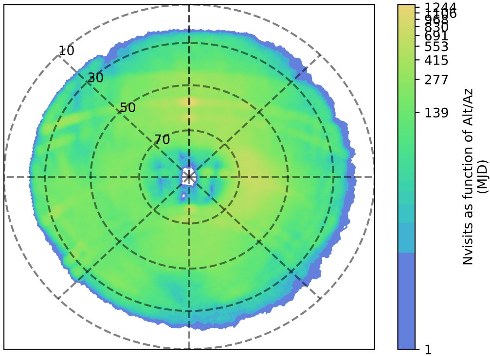
too_elab_heavy_r64_d2_ugrizy_v3.4_10yrs g: Nvisits as function of Alt/Az
