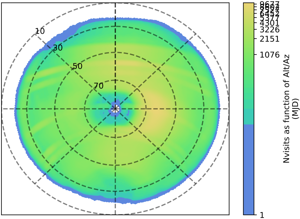
too_elab_heavy_r64_d2_ugrizy_v3.4_10yrs : Nvisits as function of Alt/Az
