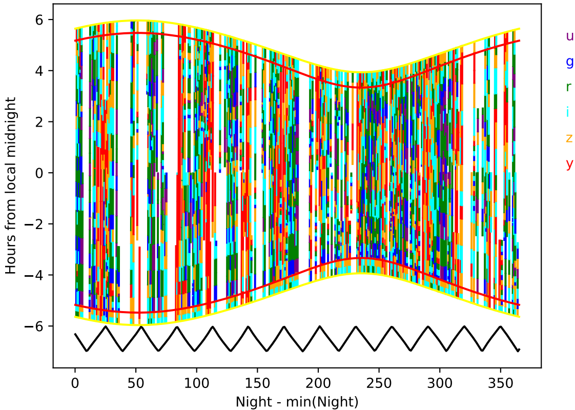
too_elab_heavy_r64_d2_ugrizy_v3.4_10yrs year 7-8: Hourglass
