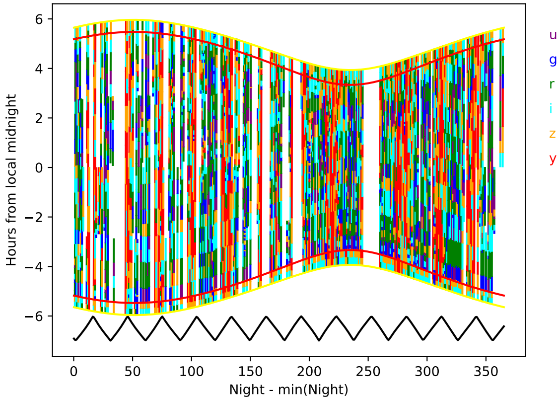
too_elab_heavy_r64_d2_ugrizy_v3.4_10yrs year 5-6: Hourglass
