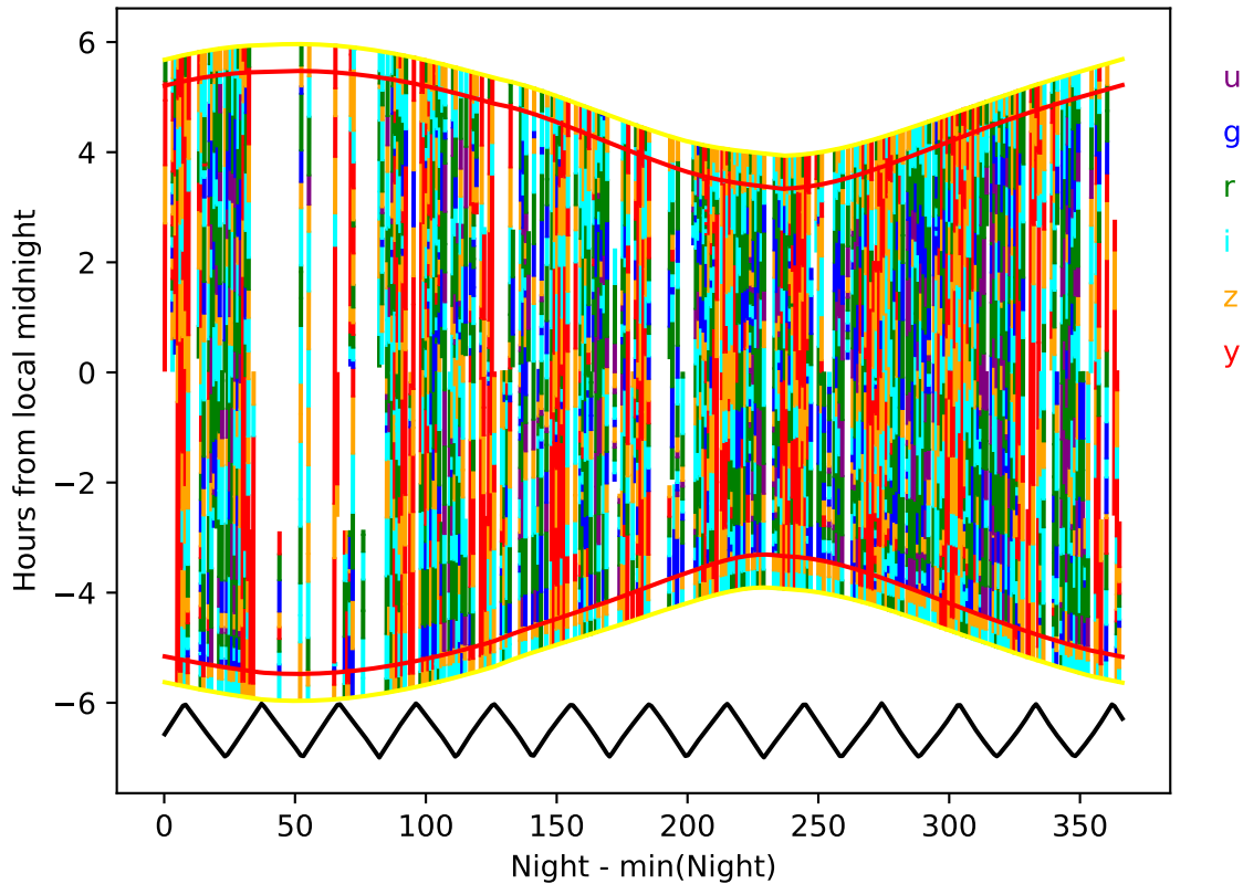
too_elab_heavy_r64_d2_ugrizy_v3.4_10yrs year 3-4: Hourglass
