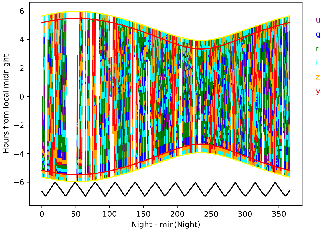
too_elab_heavy_r64_d2_ugrizy_v3.4_10yrs year 2-3: Hourglass
