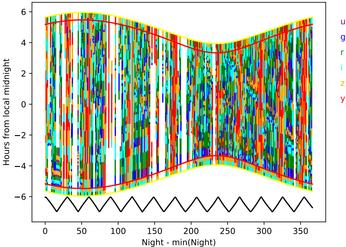
too_elab_heavy_r64_d2_ugrizy_v3.4_10yrs year 1-2: Hourglass
