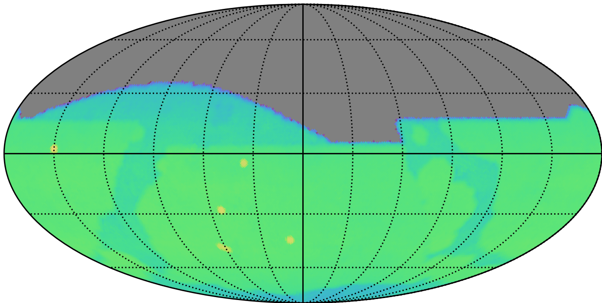
too_elab_heavy_r64_d2_ugrizy_v3.4_10yrs : CoaddM5
