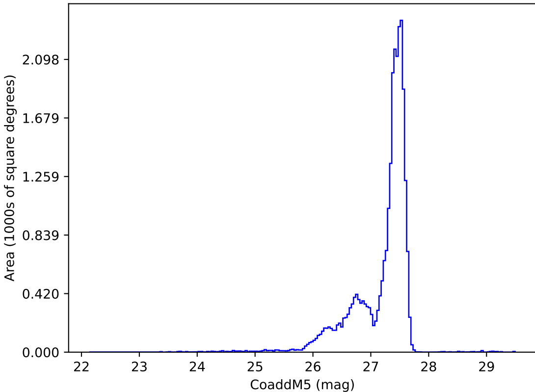
too_elab_heavy_r64_d2_ugrizy_v3.4_10yrs : CoaddM5
