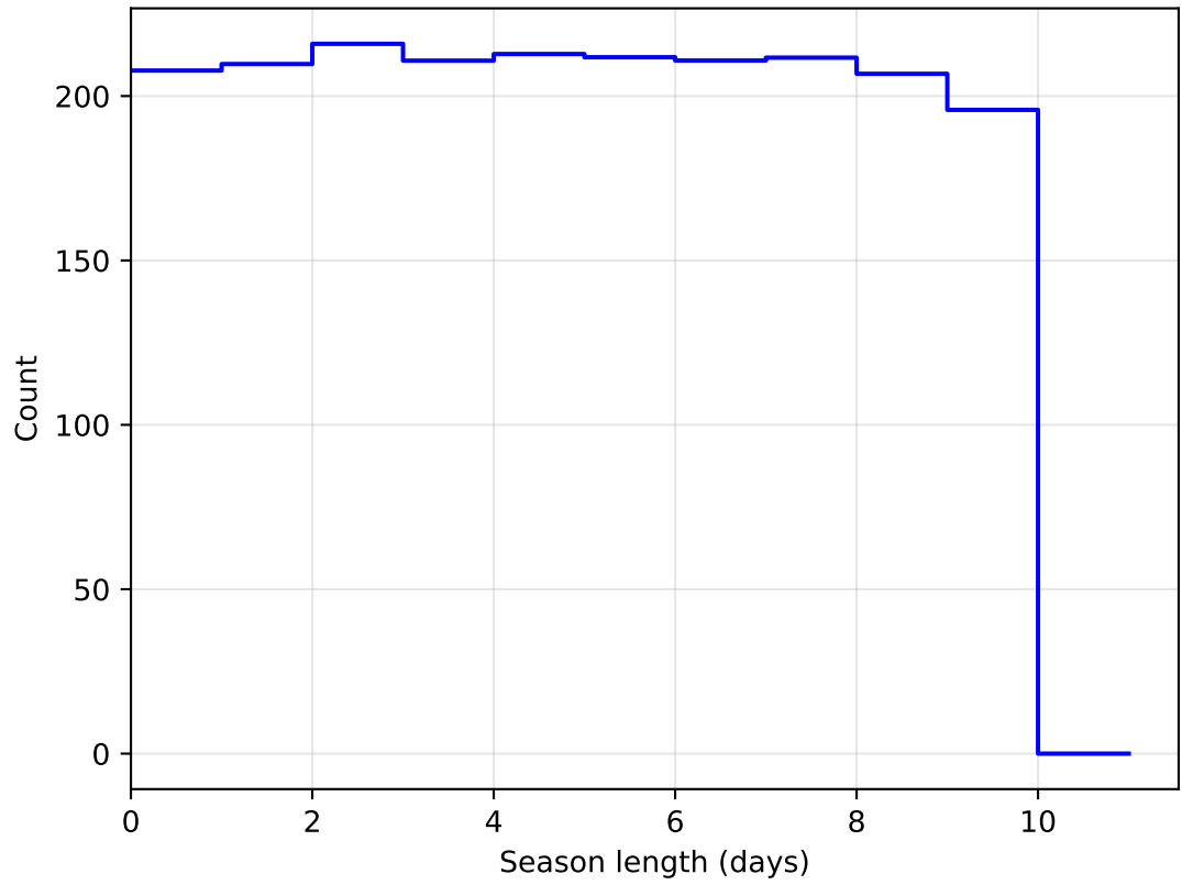
too_elab_heavy_r64_d2_ugrizy_v3.4_10yrs DD:EDFS all bands: SeasonLength
