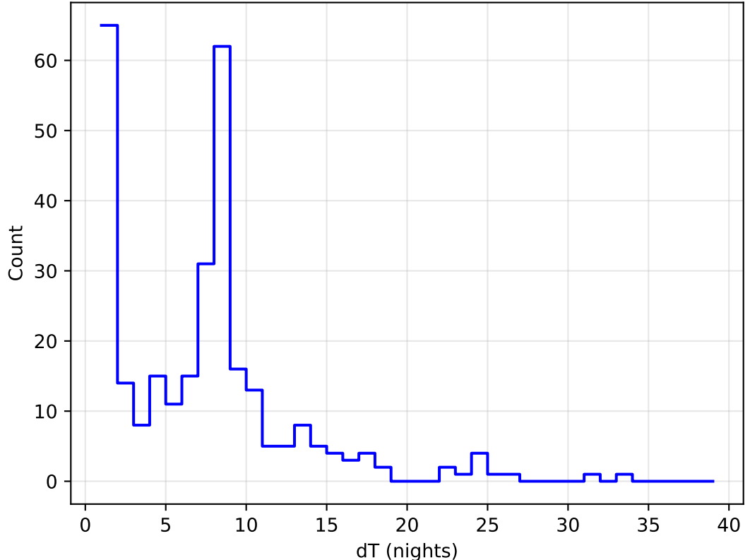
too_elab_heavy_r64_d2_ugrizy_v3.4_10yrs all bands: DD:XMM_LSS Delta Nights Histogram
