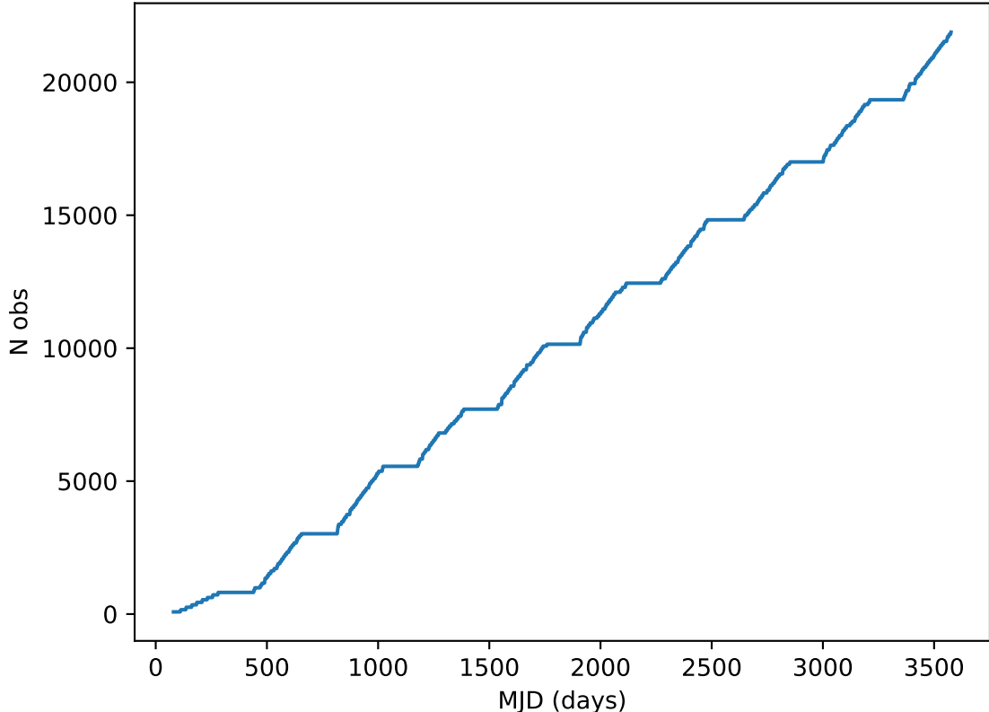
too_elab_heavy_r64_d2_ugrizy_v3.4_10yrs all bands: DD:XMM_LSS Cumulative NVisits
