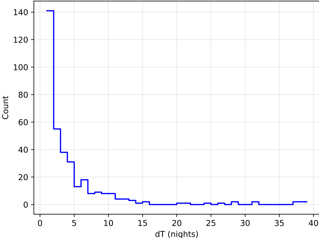
too_elab_heavy_r64_d2_ugrizy_v3.4_10yrs all bands: DD:WFD Delta Nights Histogram
