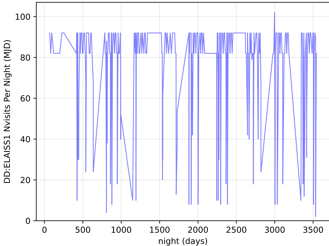
too_elab_heavy_r64_d2_ugrizy_v3.4_10yrs all bands: DD:ELAISS1 Nvisits Per Night
