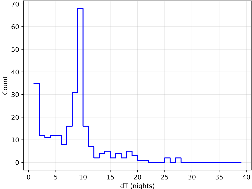
too_elab_heavy_r64_d2_ugrizy_v3.4_10yrs all bands: DD:ELAISS1 Delta Nights Histogram
