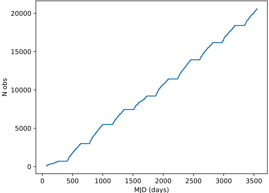
too_elab_heavy_r64_d2_ugrizy_v3.4_10yrs all bands: DD:ELAISS1 Cumulative NVisits
