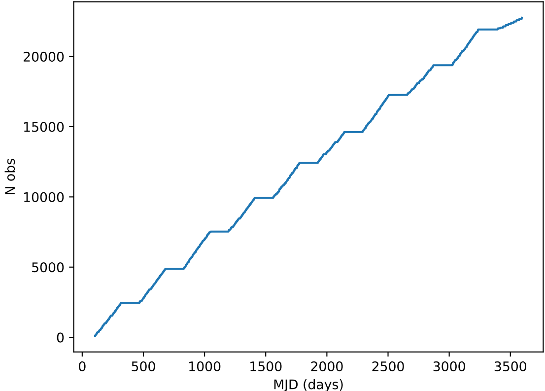
too_elab_heavy_r64_d2_ugrizy_v3.4_10yrs all bands: DD:EDFS Cumulative NVisits
