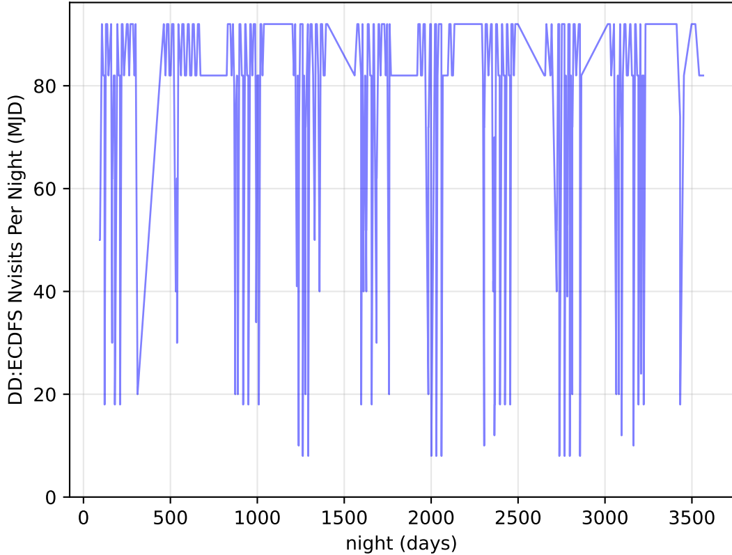
too_elab_heavy_r64_d2_ugrizy_v3.4_10yrs all bands: DD:ECDFS Nvisits Per Night
