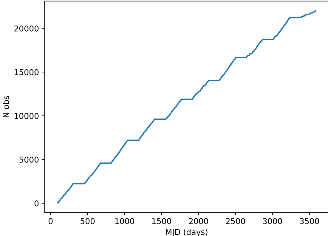
too_elab_heavy_r64_d2_ugrizy_v3.4_10yrs all bands: DD:ECDFS Cumulative NVisits
