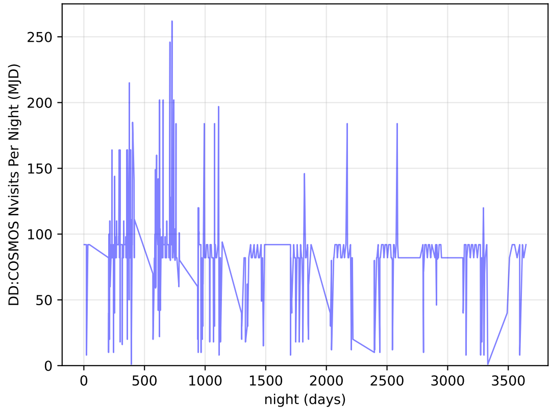
too_elab_heavy_r64_d2_ugrizy_v3.4_10yrs all bands: DD: COSMOS Nvisits Per Night
