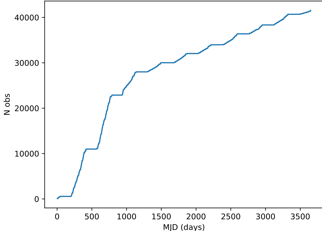
too_elab_heavy_r64_d2_ugrizy_v3.4_10yrs all bands: DD: COSMOS Cumulative NVisits
