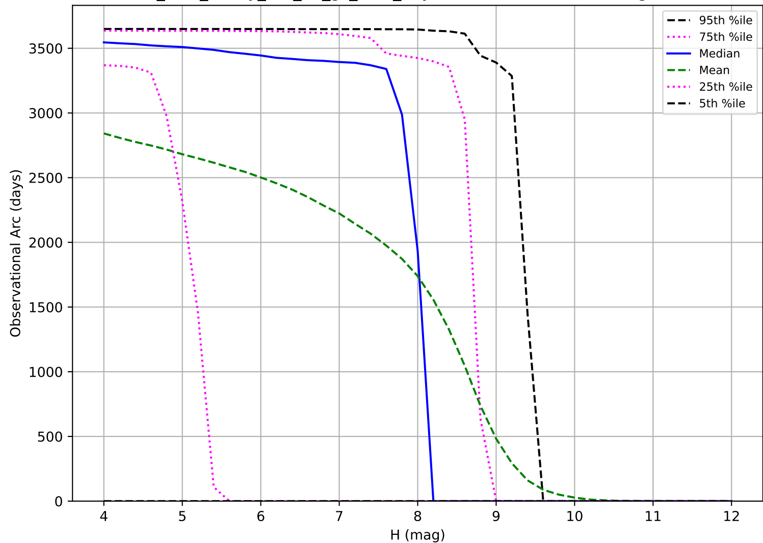
too_elab_heavy_r64_d2_gz_v3.4_10yrs: Observational Arc Length TNO
