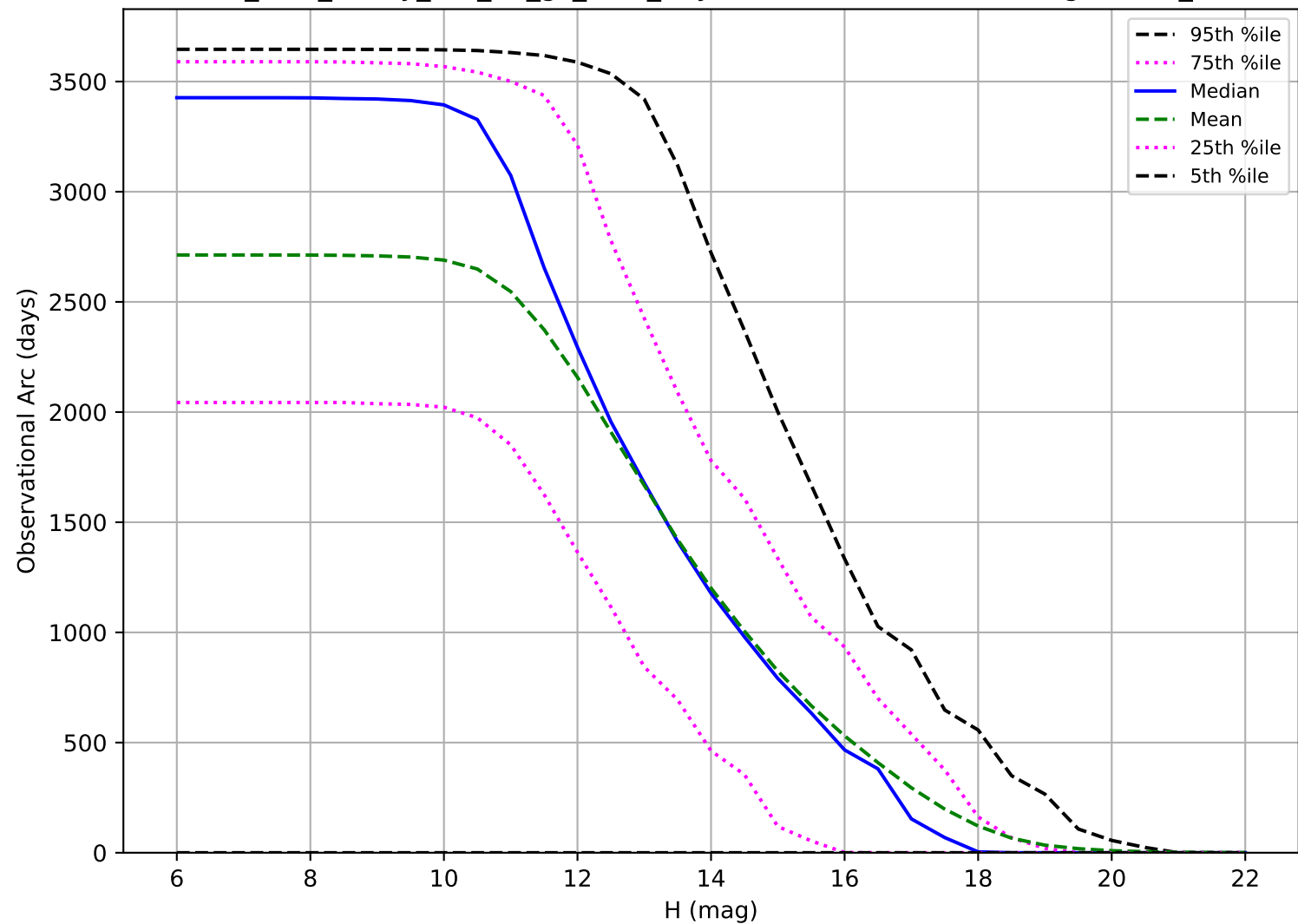
too_elab_heavy_r64_d2_gz_v3.4_10yrs: Observational Arc Length OCC_r5
