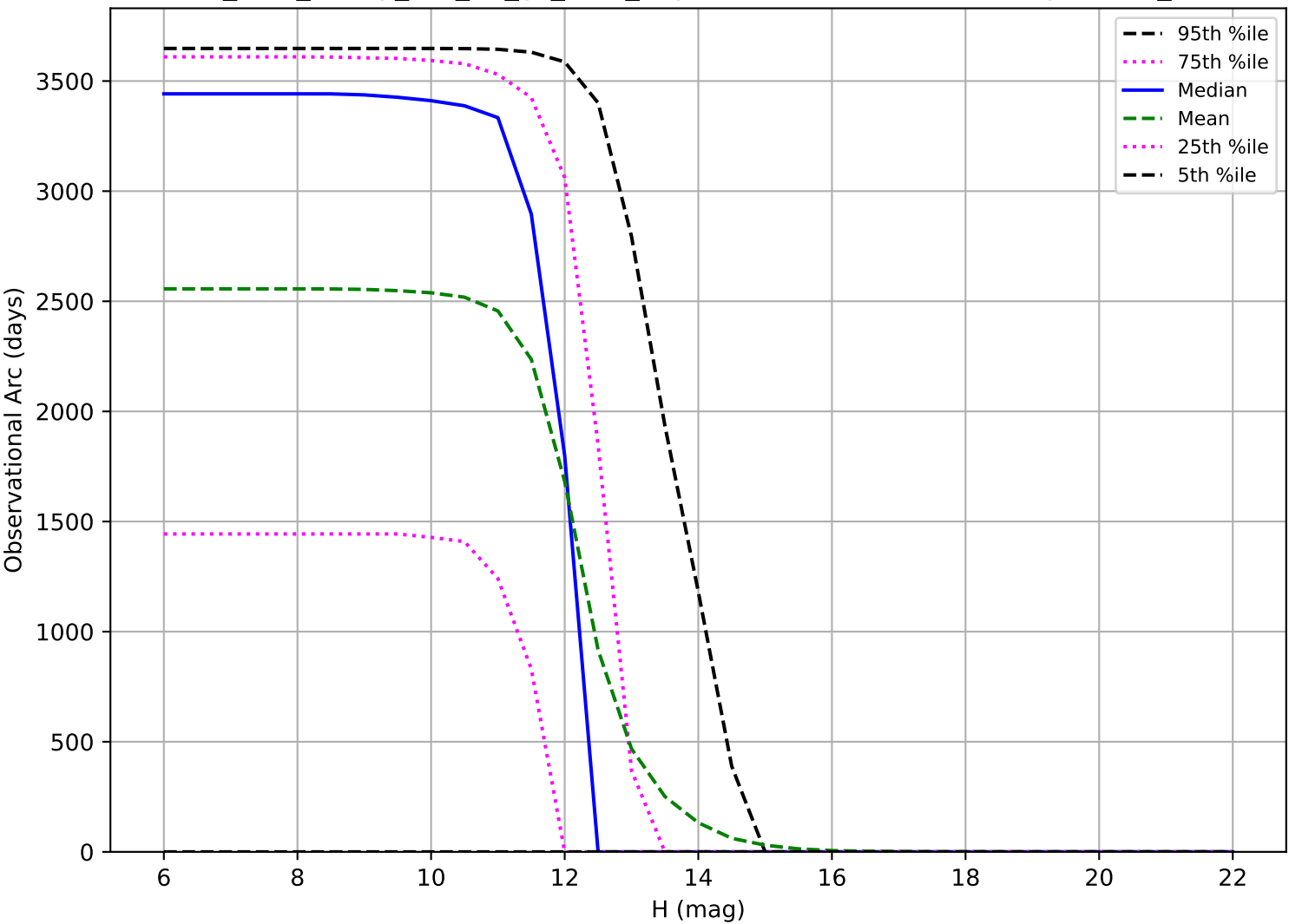
too_elab_heavy_r64_d2_gz_v3.4_10yrs: Observational Arc Length OCC_r20
