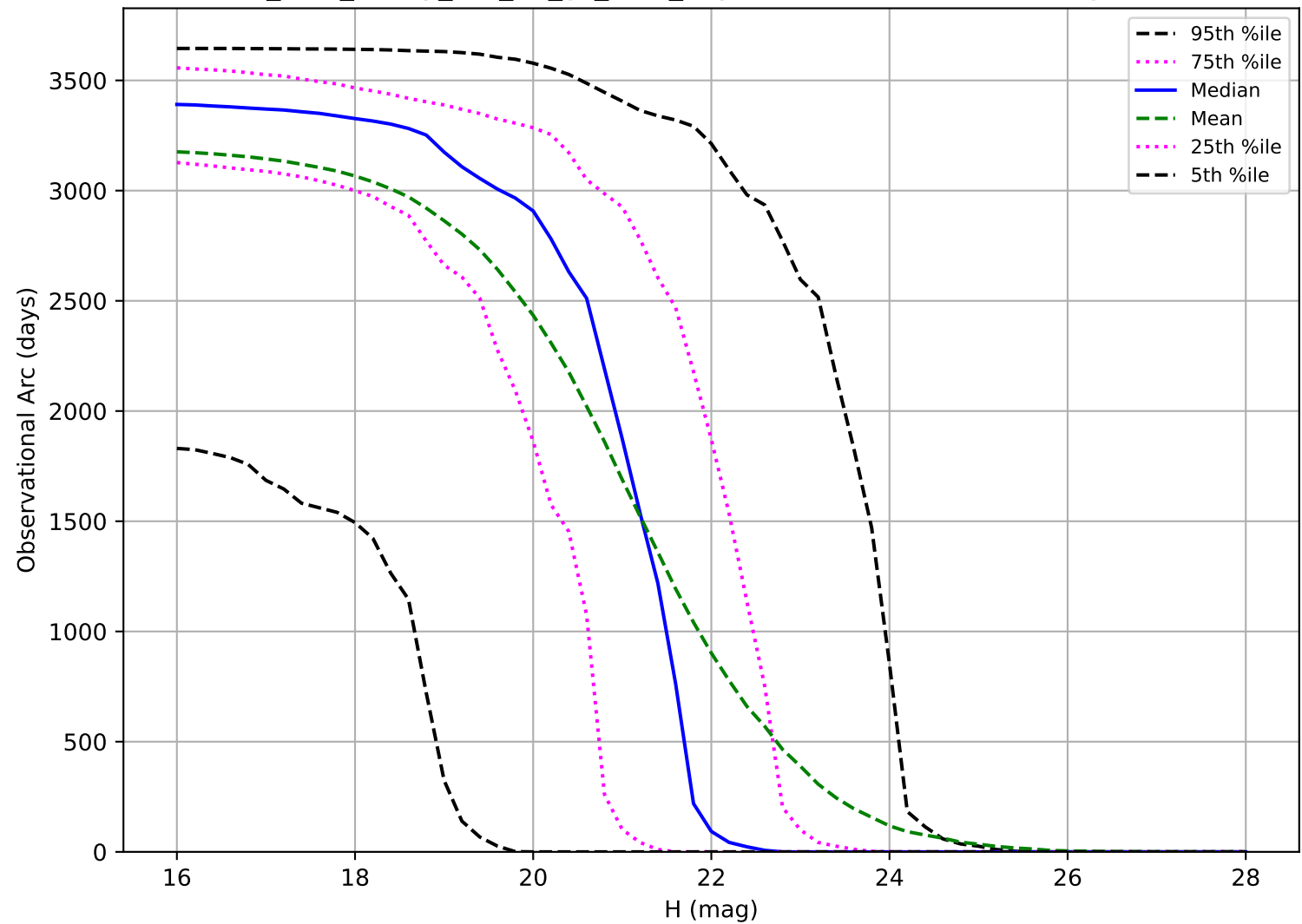
too_elab_heavy_r64_d2_gz_v3.4_10yrs: Observational Arc Length NEO
