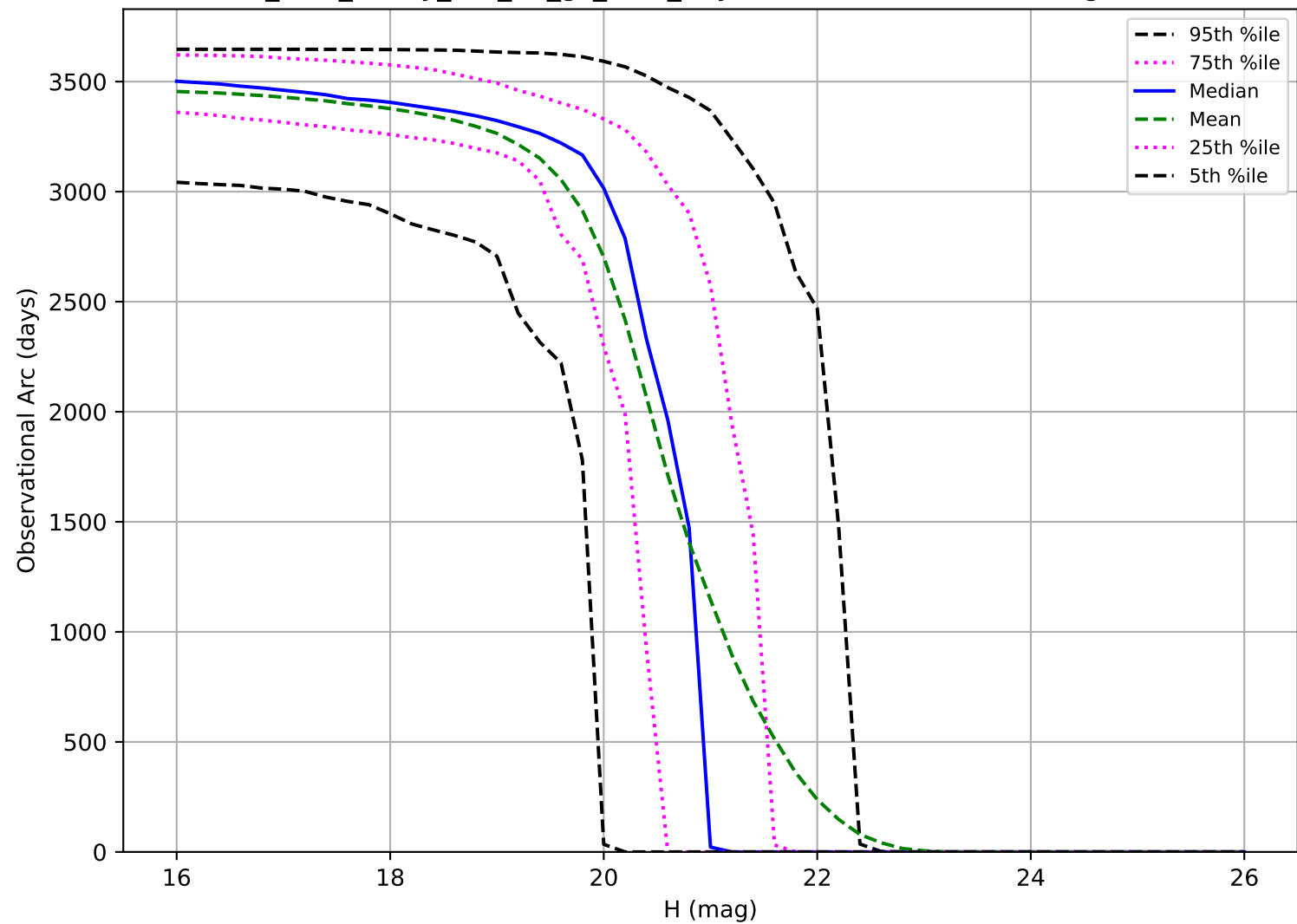
too_elab_heavy_r64_d2_gz_v3.4_10yrs: Observational Arc Length MBA
