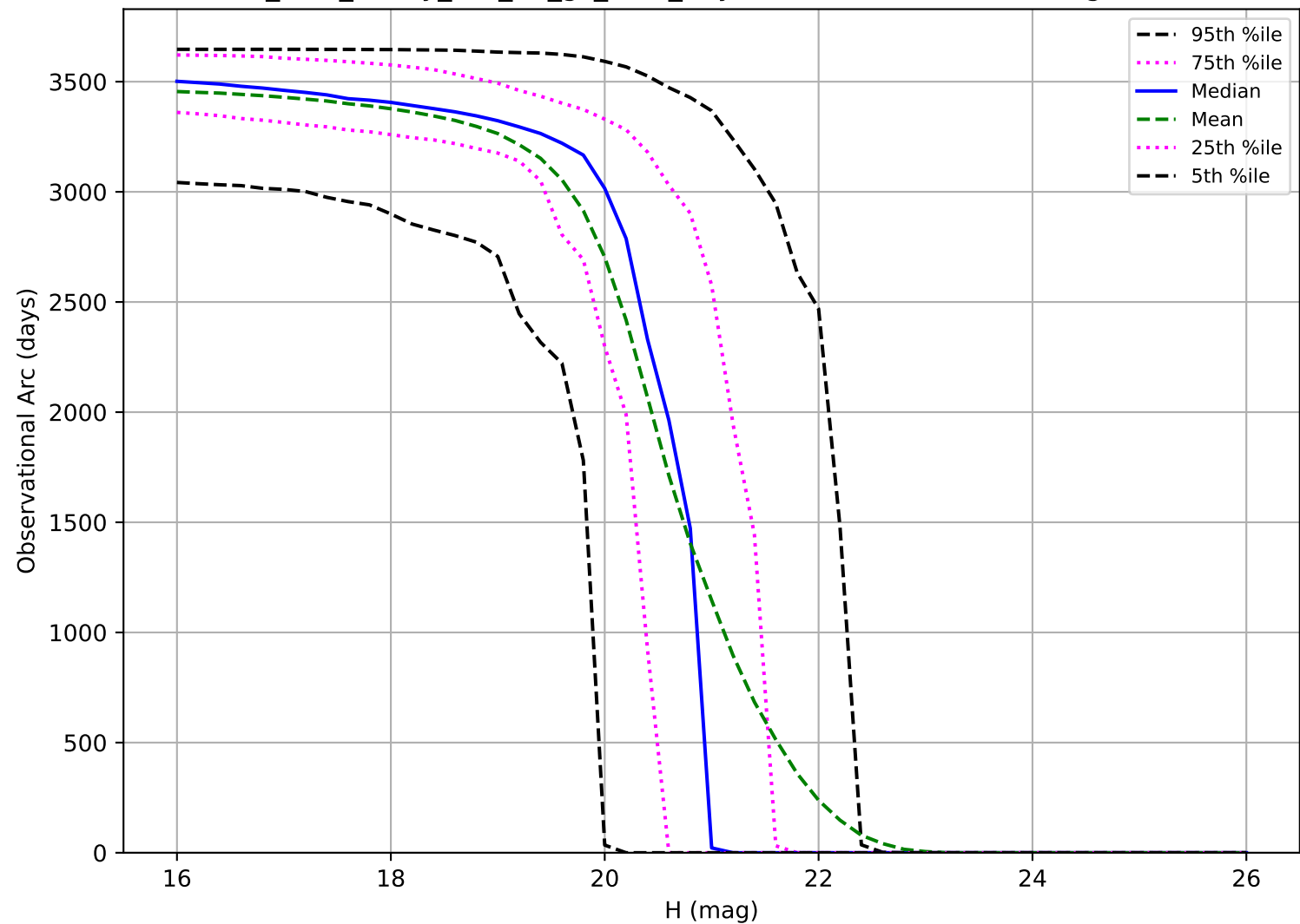
too_elab_heavy_r64_d2_gz_v3.4_10yrs: Observational Arc Length MBA
