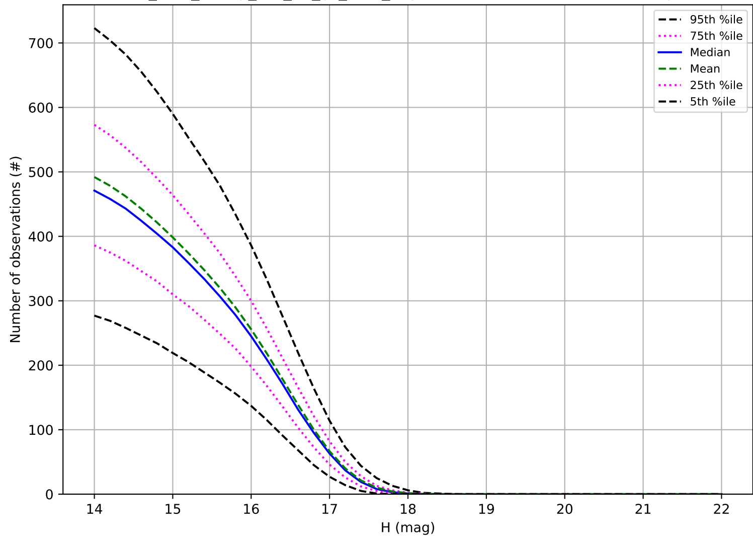
too_elab_heavy_r64_d2_gz_v3.4_10yrs: Number of observations Trojan
