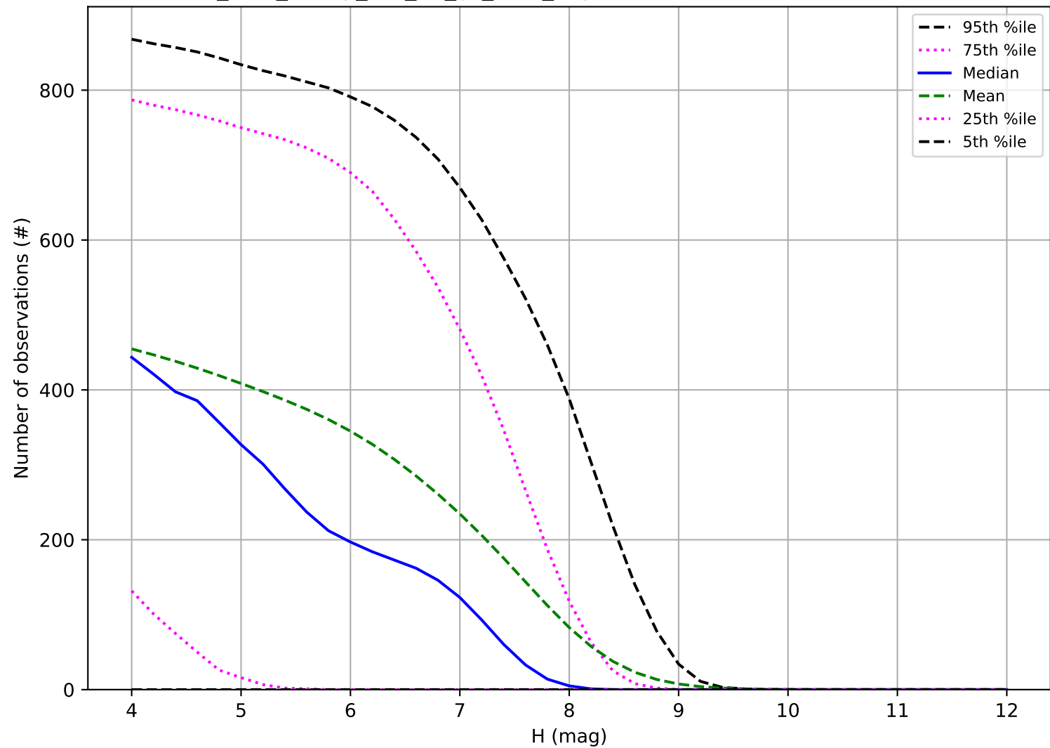
too_elab_heavy_r64_d2_gz_v3.4_10yrs: Number of observations TNO
