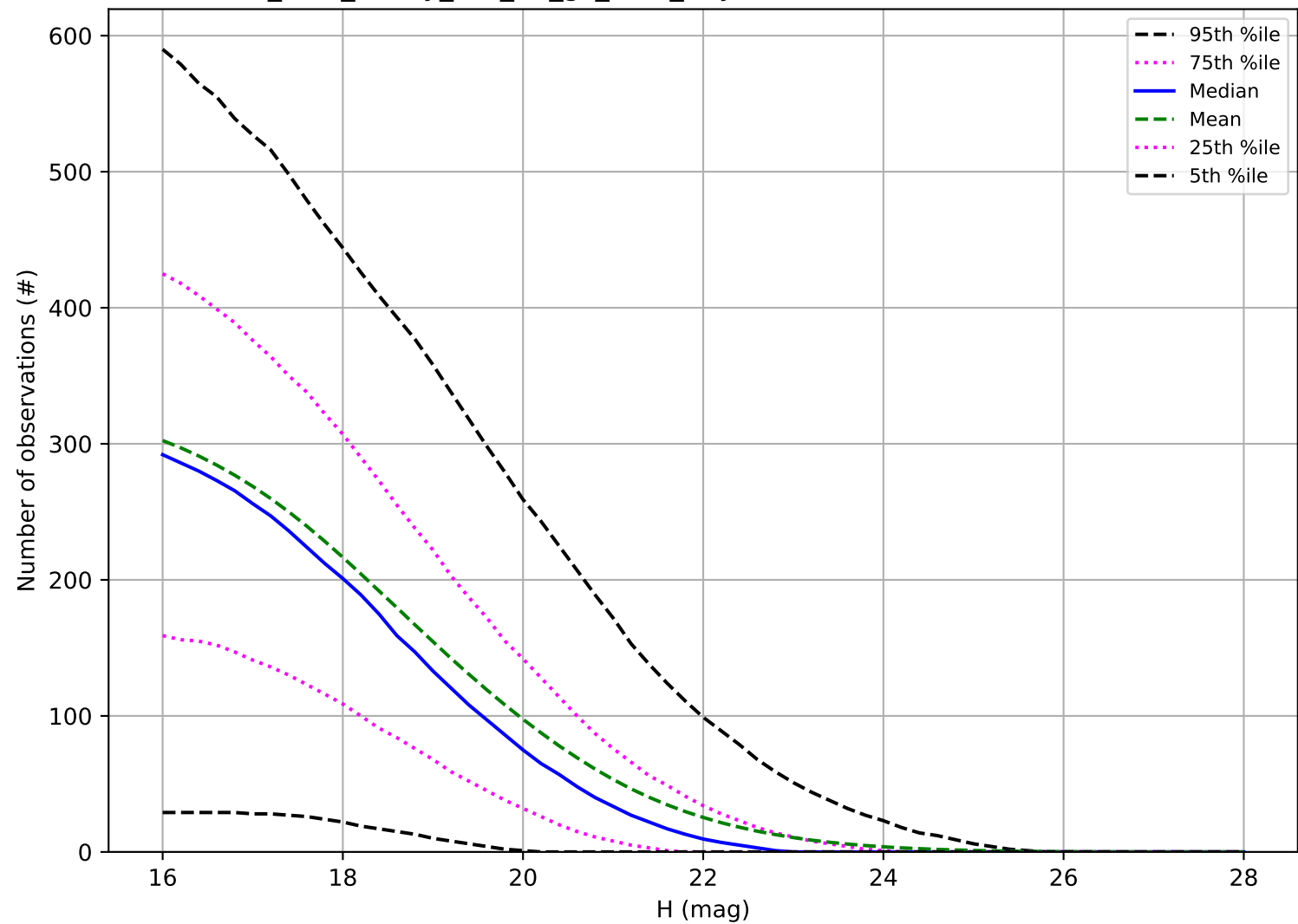
too_elab_heavy_r64_d2_gz_v3.4_10yrs: Number of observations NEO
