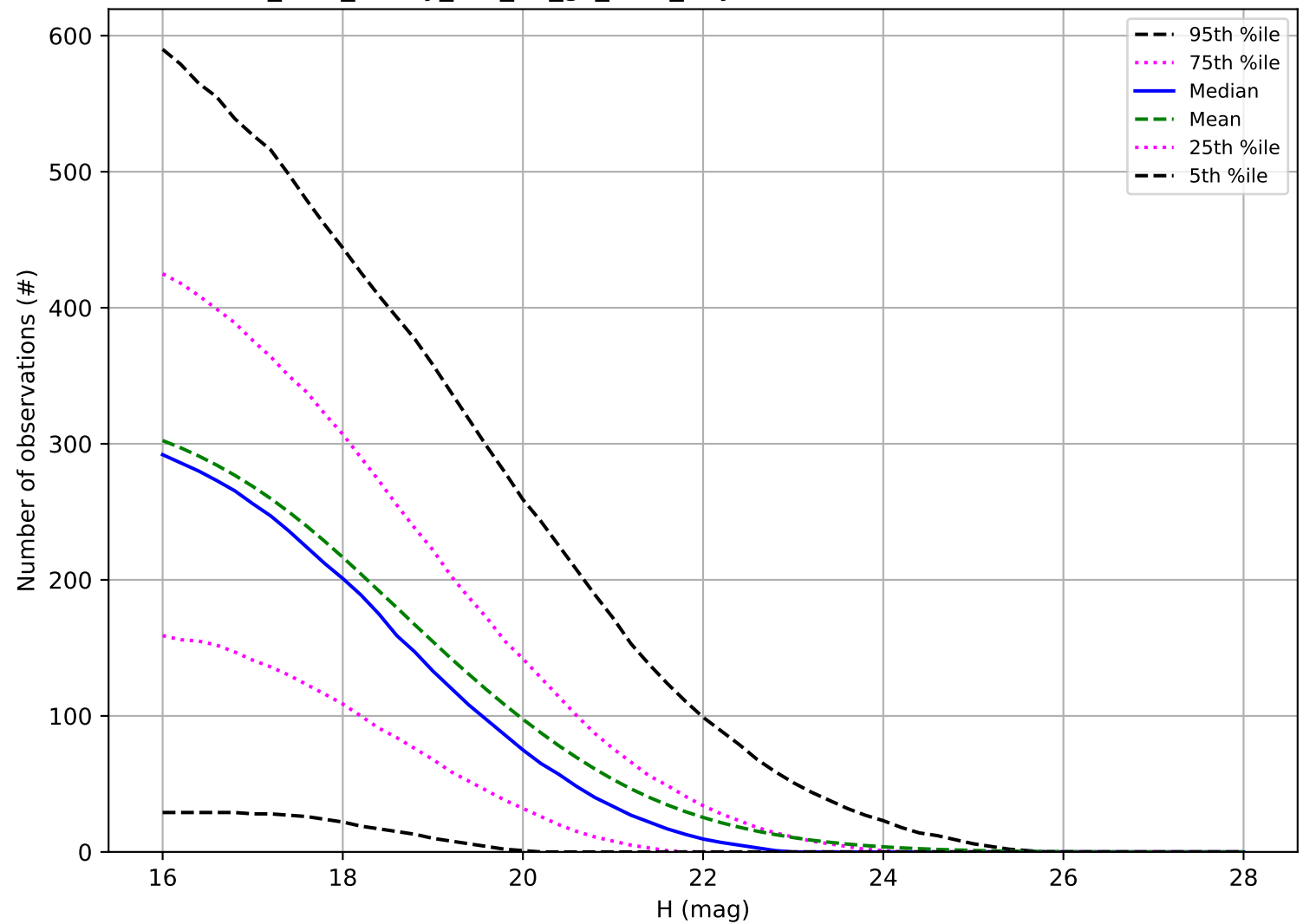
too_elab_heavy_r64_d2_gz_v3.4_10yrs: Number of observations NEO
