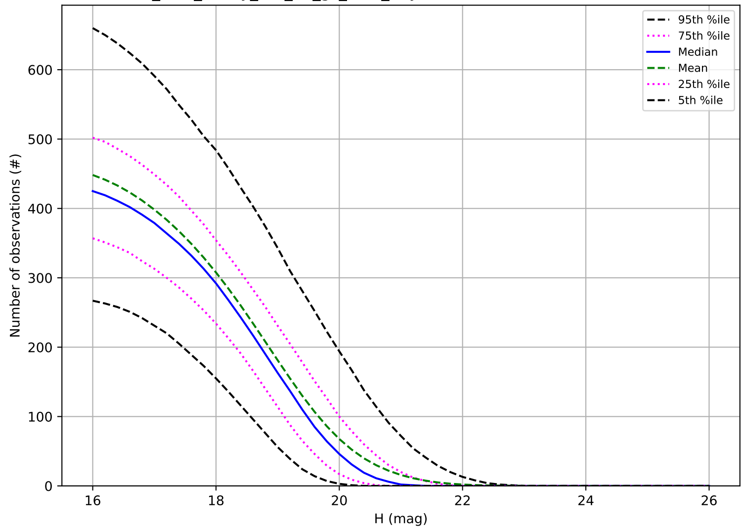
too_elab_heavy_r64_d2_gz_v3.4_10yrs: Number of observations MBA
