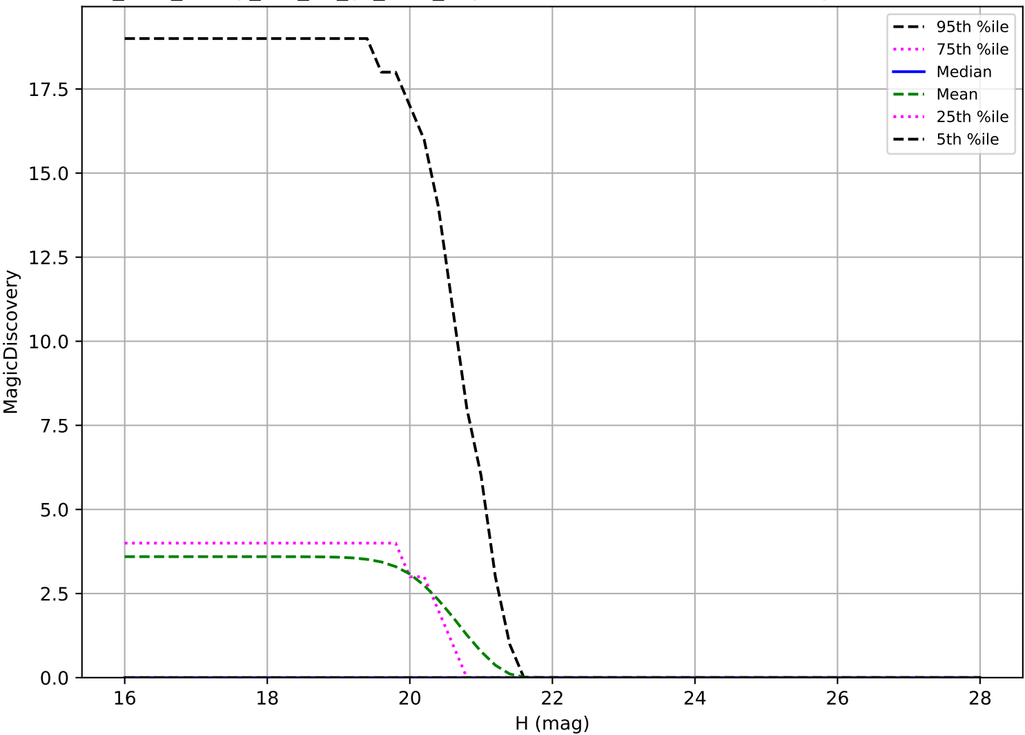
too_elab_heavy_r64_d2_gz_v3.4_10yrs: Vatira 6 detections in 60 nights detection loss
