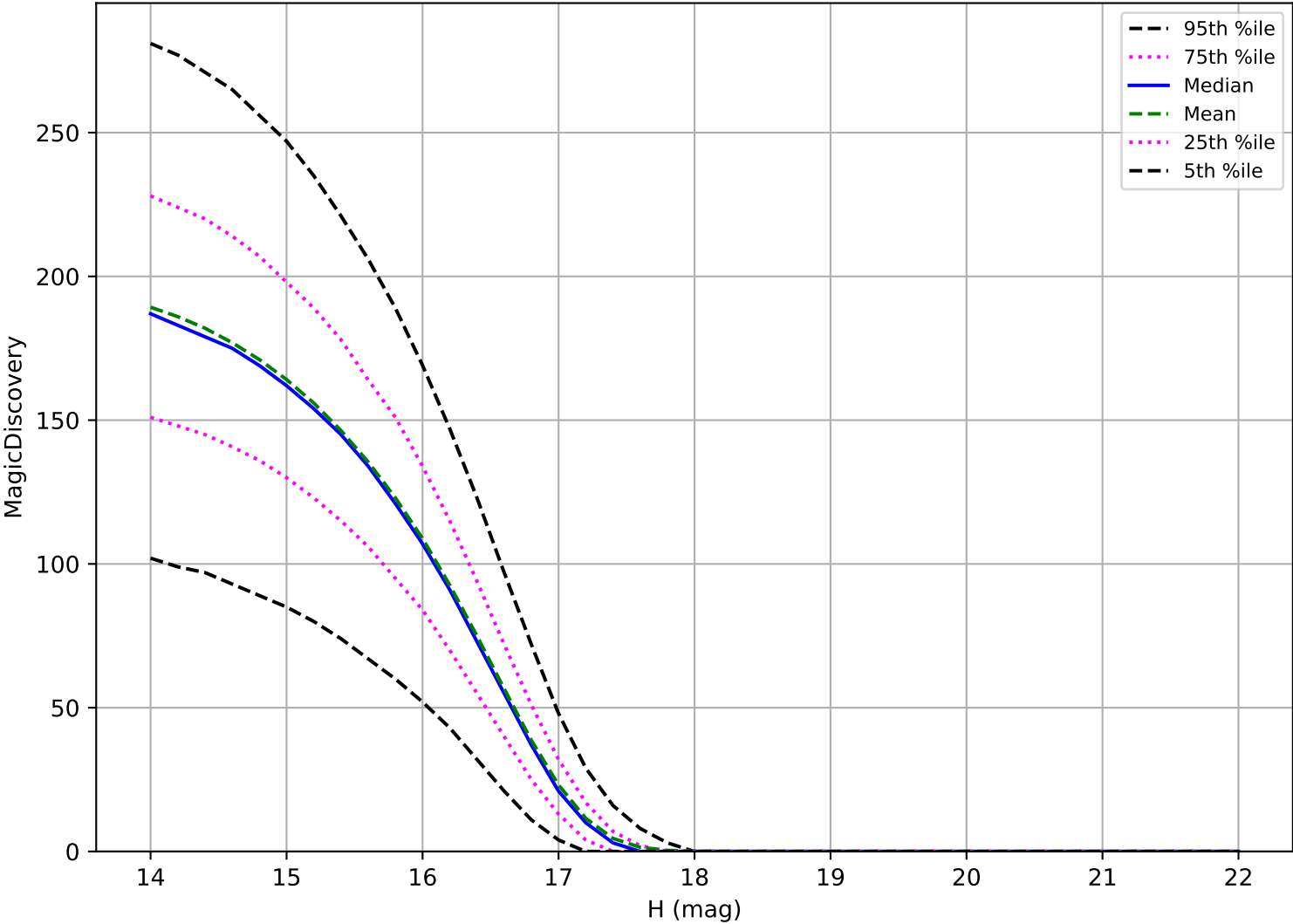
too_elab_heavy_r64_d2_gz_v3.4_10yrs: Trojan 6 detections in 60 nights detection loss
