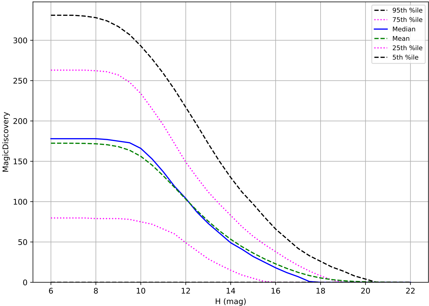
too_elab_heavy_r64_d2_gz_v3.4_10yrs: OCC_r5 6 detections in 60 nights detection loss
