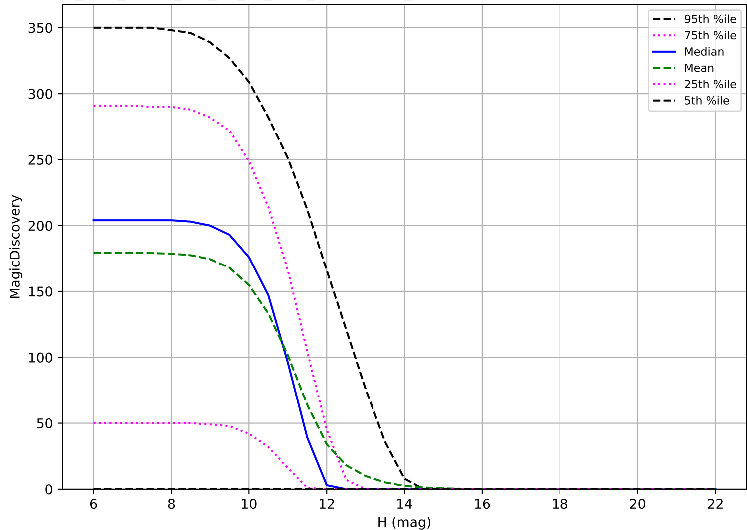
too_elab_heavy_r64_d2_gz_v3.4_10yrs: OCC_r20 6 detections in 60 nights detection loss
