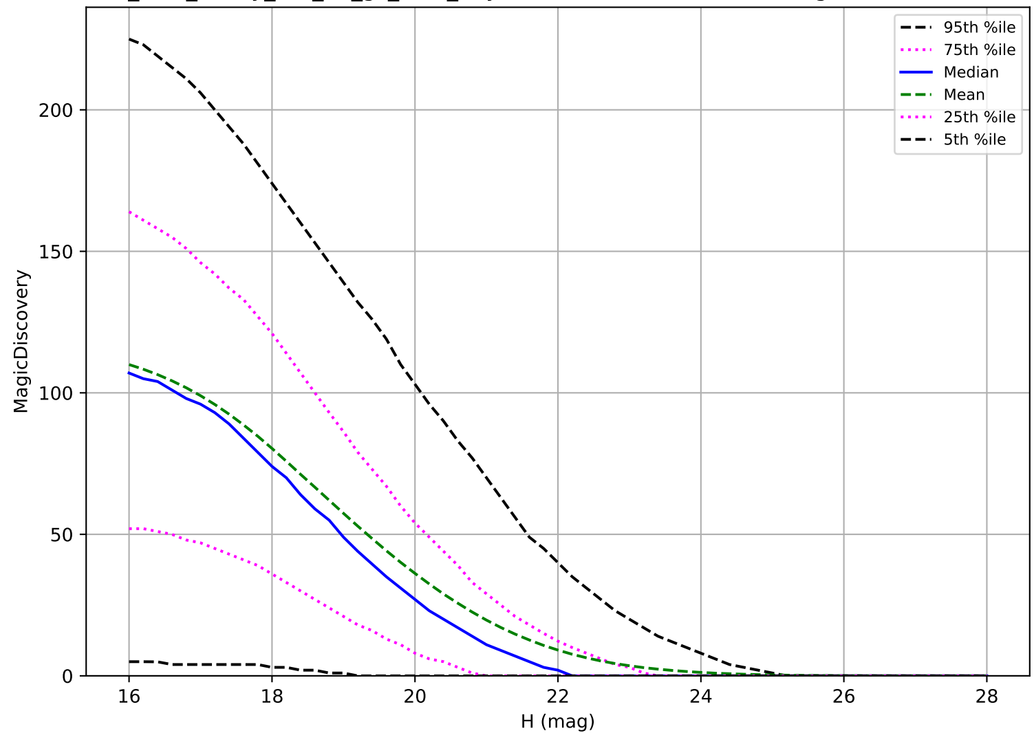
too_elab_heavy_r64_d2_gz_v3.4_10yrs: NEO 6 detections in 60 nights detection loss
