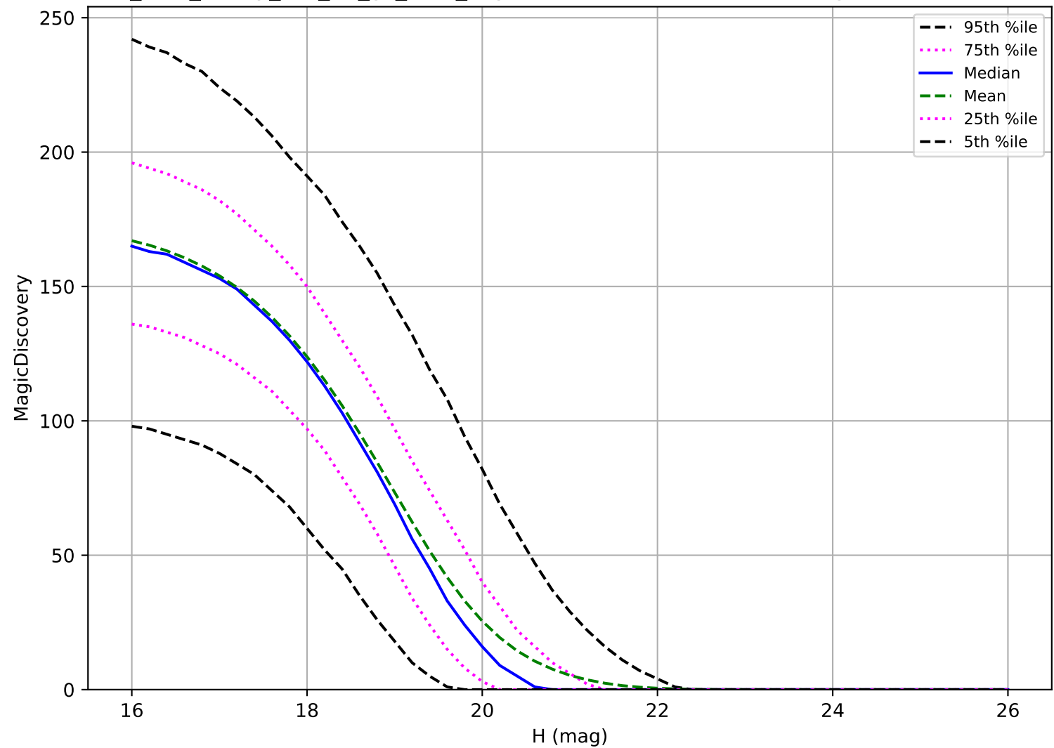
too_elab_heavy_r64_d2_gz_v3.4_10yrs: MBA 6 detections in 60 nights detection loss
