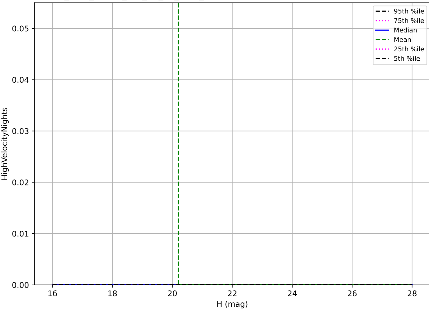
too_elab_heavy_r64_d2_gz_v3.4_10yrs: Vatira High velocity pair detection loss
