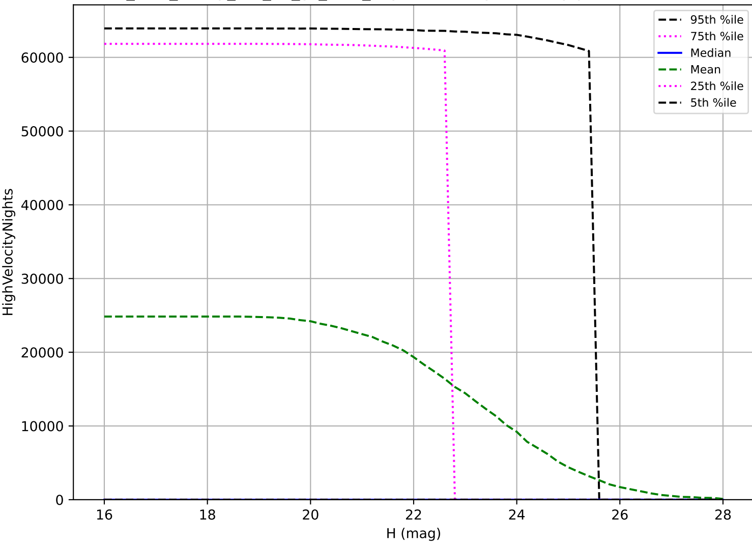
too_elab_heavy_r64_d2_gz_v3.4_10yrs: PHA High velocity pair detection loss
