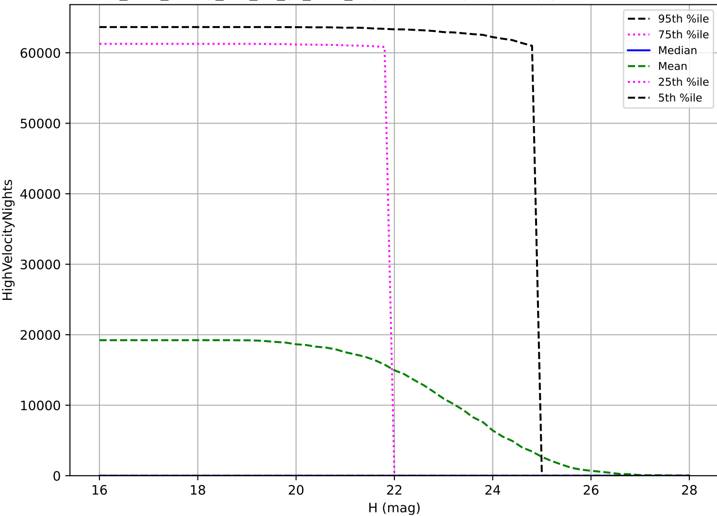
too_elab_heavy_r64_d2_gz_v3.4_10yrs: NEO High velocity pair detection loss
