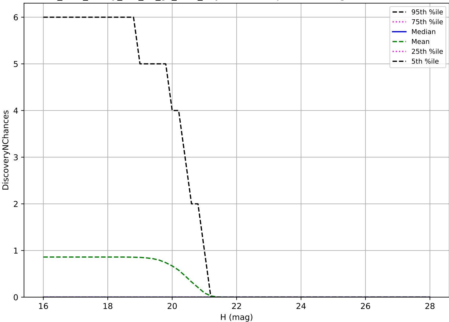
too_elab_heavy_r64_d2_gz_v3.4_10yrs: Vatira 3 pairs in 15 nights detection loss
