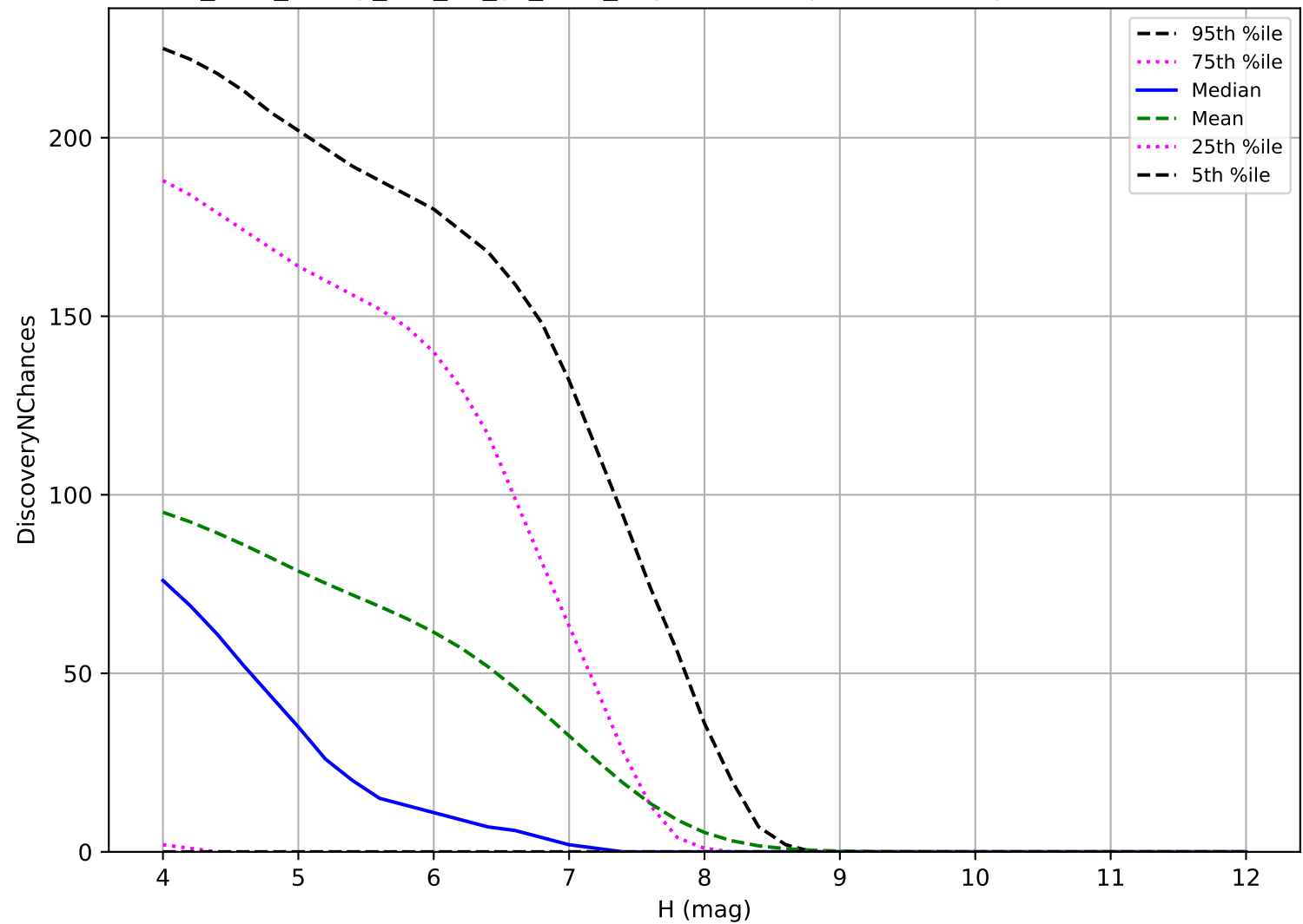
too_elab_heavy_r64_d2_gz_v3.4_10yrs: TNO 3 pairs in 15 nights detection loss
