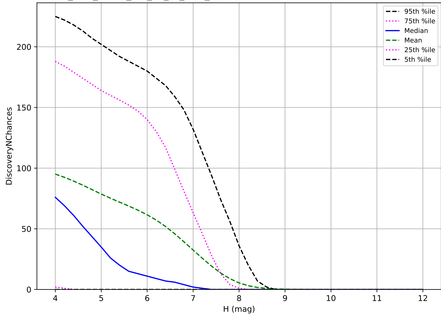
too_elab_heavy_r64_d2_gz_v3.4_10yrs: TNO 3 pairs in 15 nights detection loss
