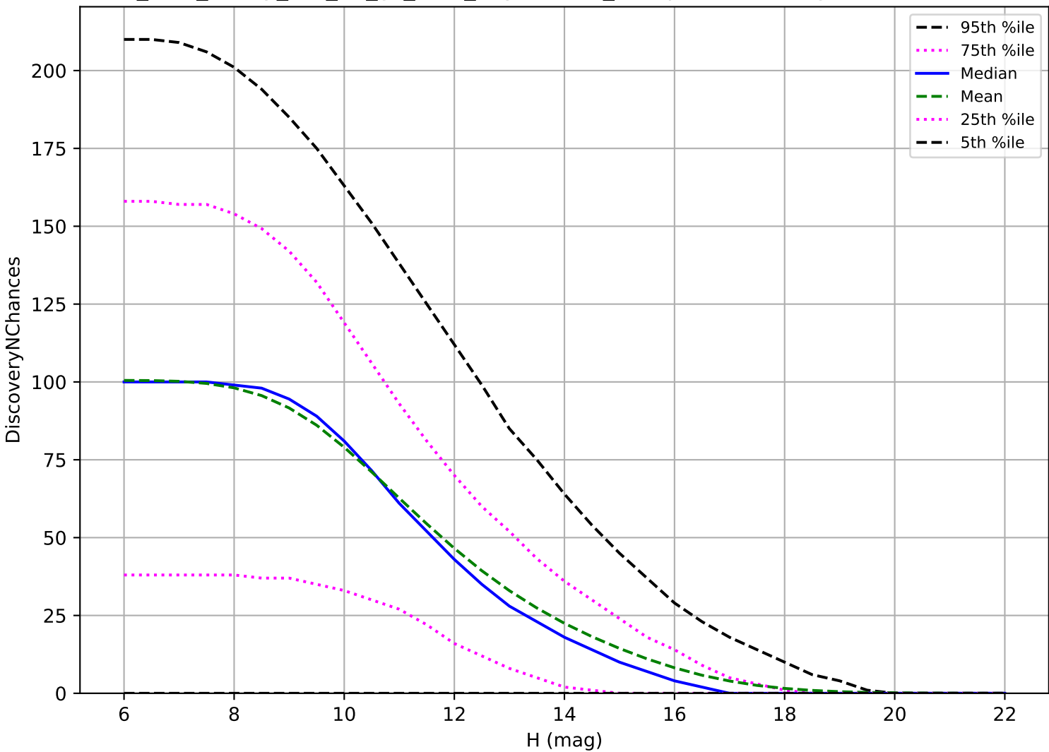
too_elab_heavy_r64_d2_gz_v3.4_10yrs: OCC_r5 3 pairs in 15 nights detection loss
