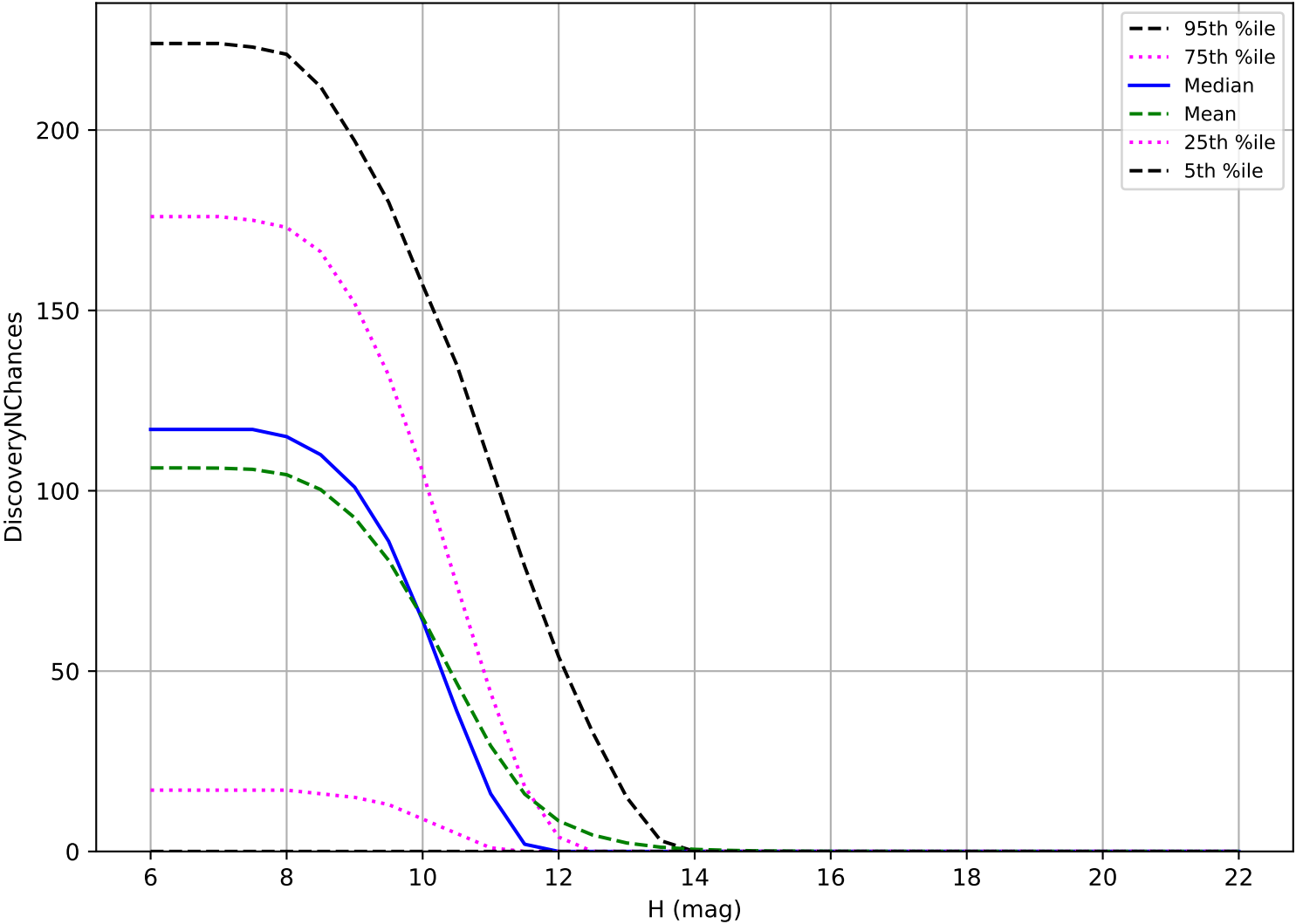
too_elab_heavy_r64_d2_gz_v3.4_10yrs: OCC_r20 3 pairs in 15 nights detection loss
