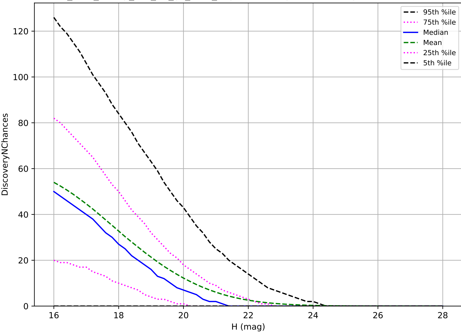
too_elab_heavy_r64_d2_gz_v3.4_10yrs: NEO 3 pairs in 15 nights detection loss
