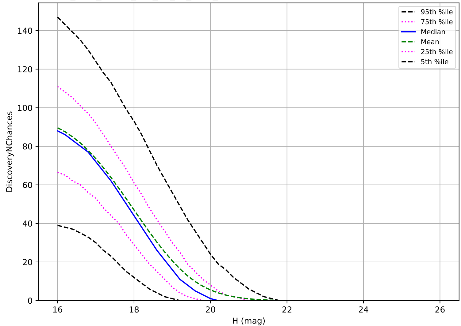
too_elab_heavy_r64_d2_gz_v3.4_10yrs: MBA 3 pairs in 15 nights detection loss
