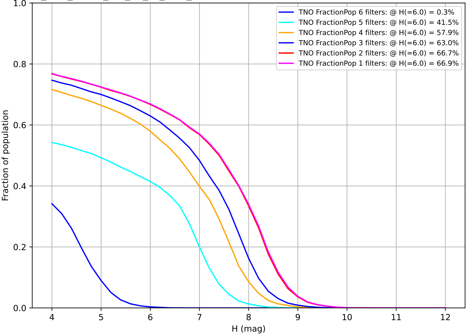
too_elab_heavy_r64_d2_gz_v3.4_10yrs: Fraction of population with colors in X filters TNO
