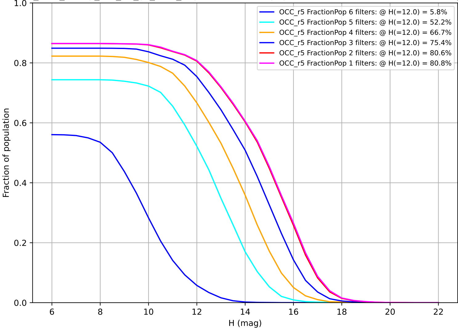
too_elab_heavy_r64_d2_gz_v3.4_10yrs: Fraction of population with colors in X filters OCC_r5
