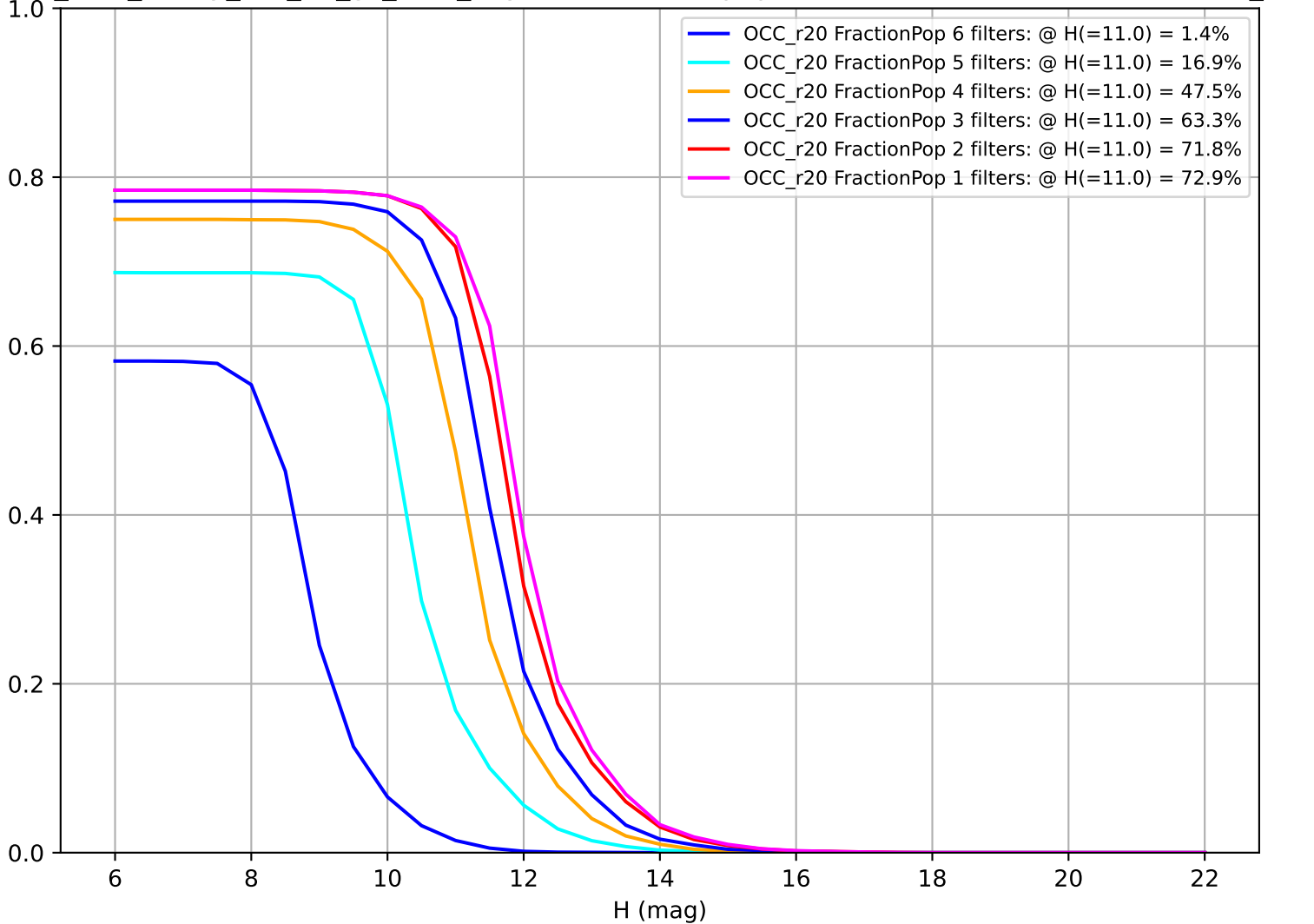
too_elab_heavy_r64_d2_gz_v3.4_10yrs: Fraction of population with colors in X filters OCC_r20
